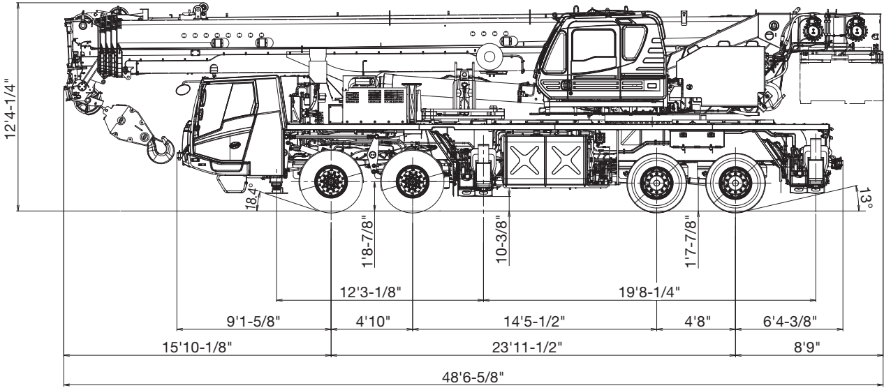
Dimension is with boom angle at -0.4 degree.
