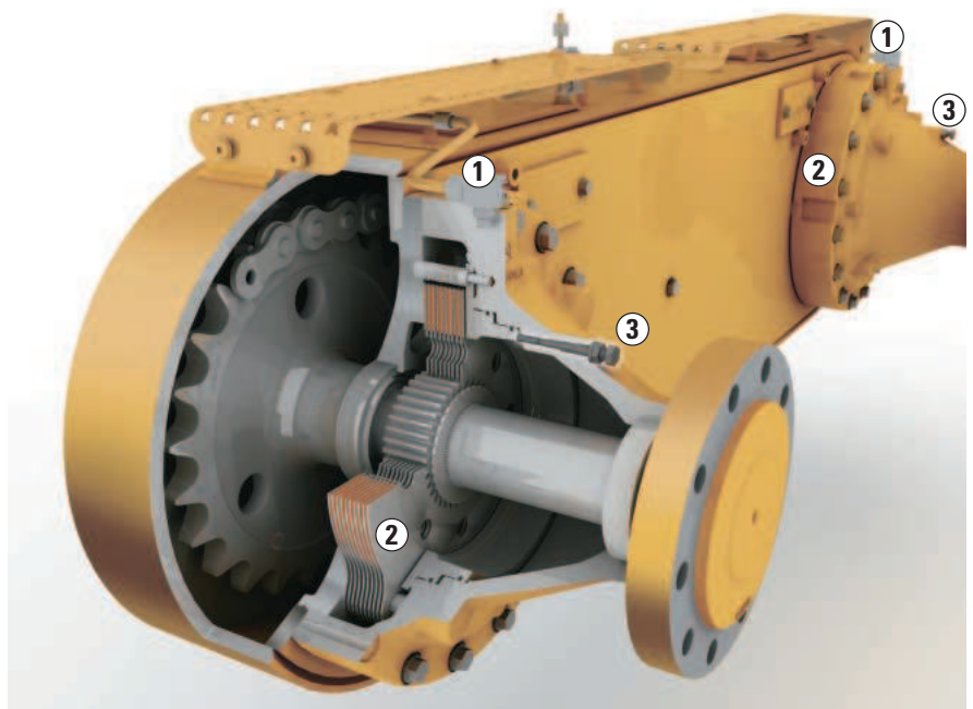
Brake design
