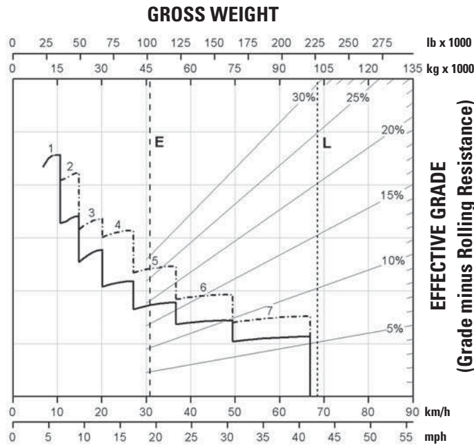
Grade Distance – 600 m (2,000 ft)
