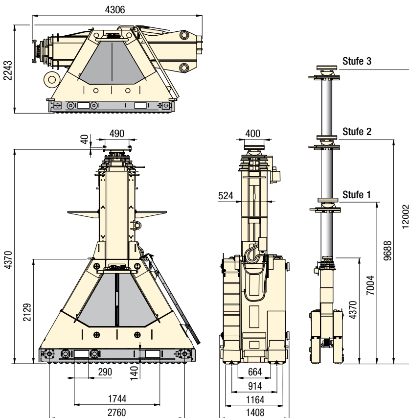
Abmessungen in mm.
