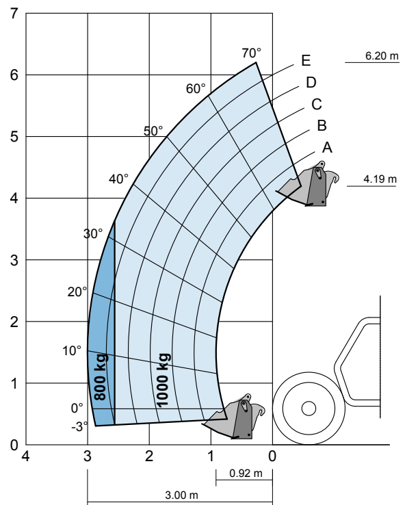
On tyres with 4-in-1 bucket 500 L
