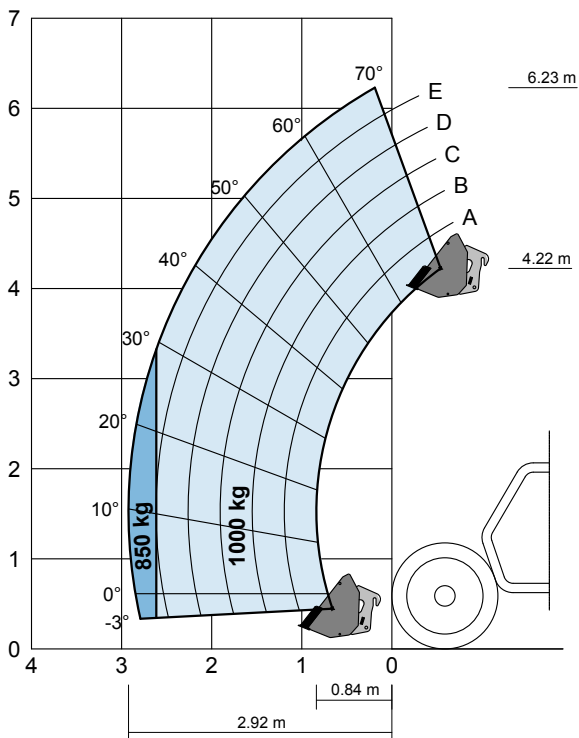
On tyres with 500 L GP bucket
