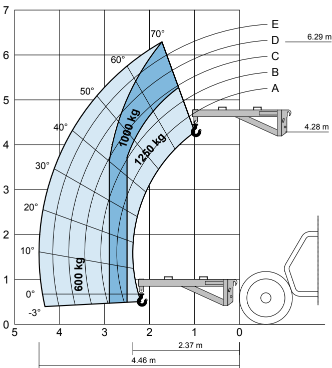
On tyres with 2m jib
