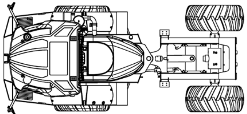
The MultiChassis seen from above. Here the 912D MultiChassis, ready for add-on-tools.
