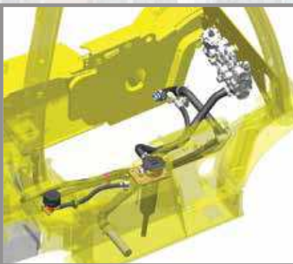
Hydraulic System
