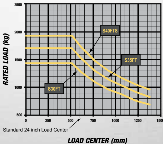
RATED LOAD vs. LOAD CENTER INTEGRAL CARRIAGE METRIC
