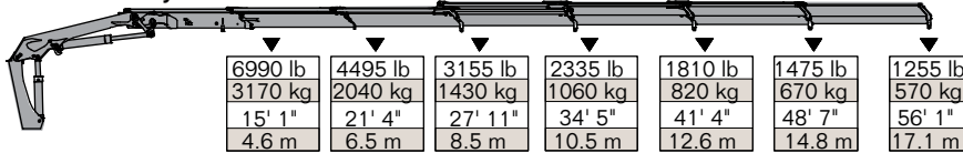
18/124SL - 6 Hydraulic
