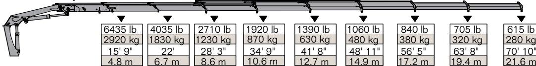
18/124SL - 8 Hydraulic
