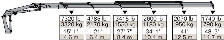
18/124SL - 5 Hydraulic
