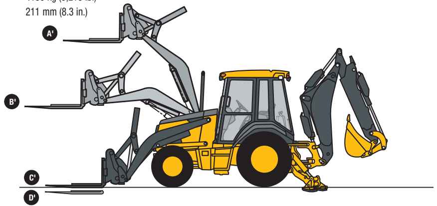
410J TMC Backhoe with 1.22-m (4 ft.) Extendable Dipperstick, Retracted
