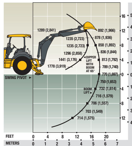
310J Backhoe with 1.07-m (3 ft. 6 in.) Extendable Dipperstick, Extended
