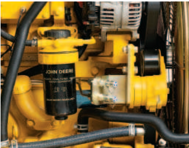
Vertical spin-on engine, transmission, and hydraulic filters and quick-release fuel filters allow quick, no-spill changes.
