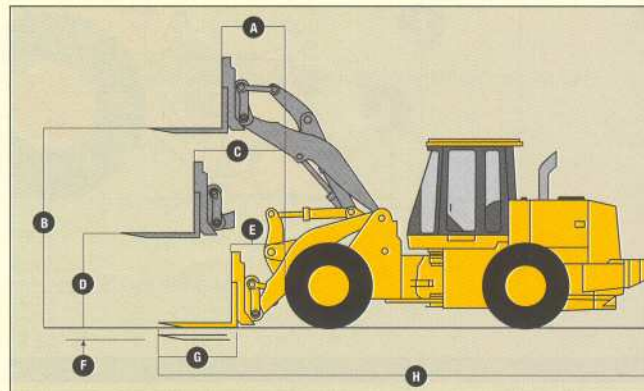
644H LOADER WITH QUICK-COUPLER AND PALLET FORK*
