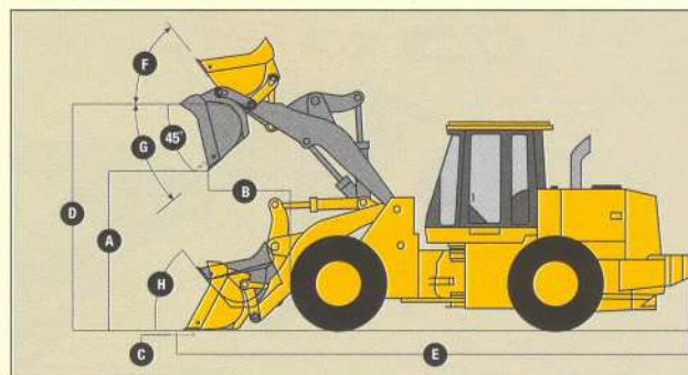
644H LOADER WITH QUICK-COUPLER AND BUCKET*
