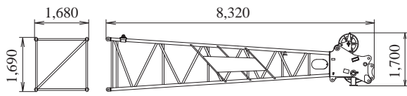
Boom Tip Weight: 1,535 kg
