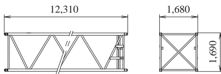
12.2 m Boom Insert Weight: 1,195 kg
