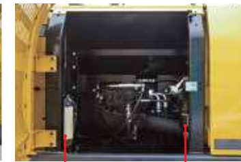
Fuel Filter (with built-in water separator) Engine Oil Filter
