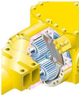
Service Brakes
