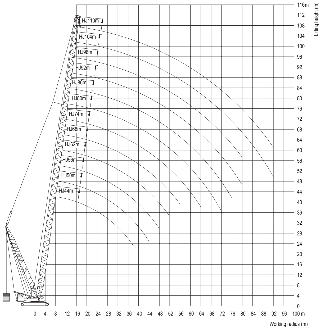
Working range curve
