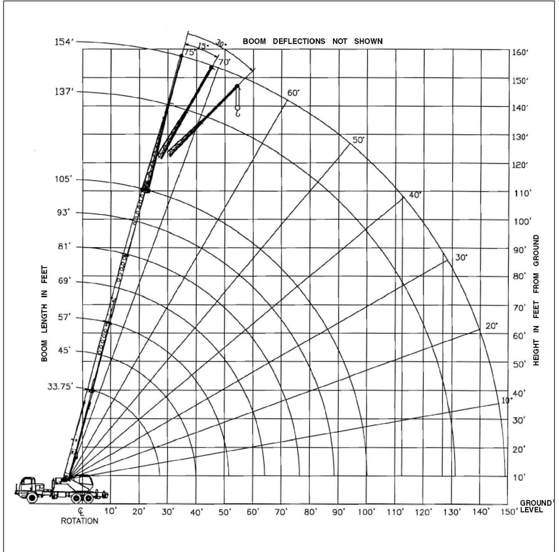
Range Diagram (33.75' - 105' boom)
