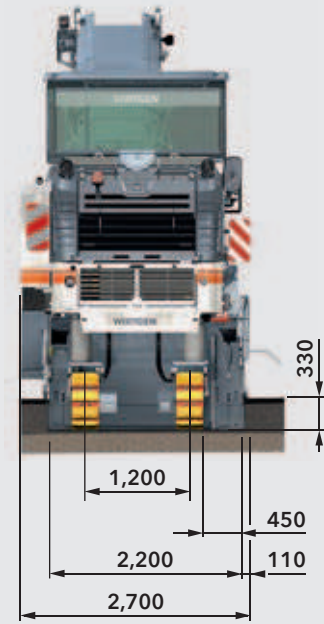
W 210/W 210i with 2.2-m drum assembly
